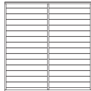
5 Internal Panel QTY 1 1712mm x 1760mm AI-S21SHPPTOV1712X1760-V1
