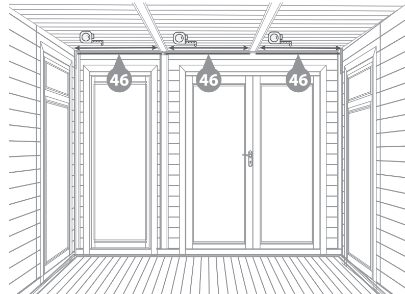
*Internal view of the front wall*
