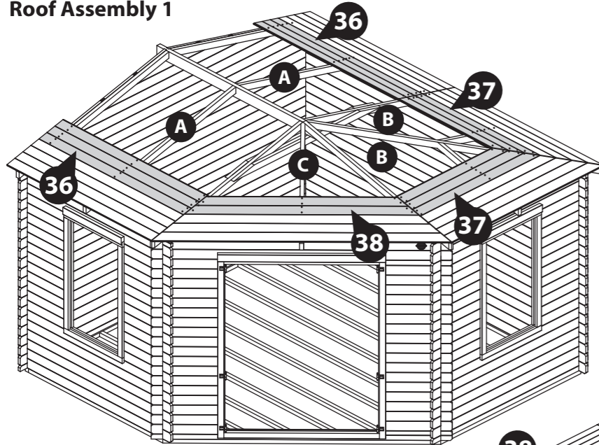
Roof Assembly 1
