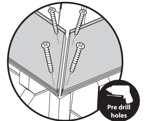
Roof Assembly 2
