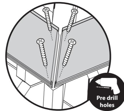
Roof Assembly 2
