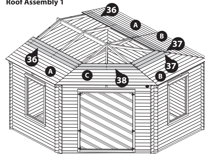
Roof Assembly 1
