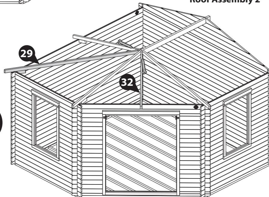
Roof Assembly 2
