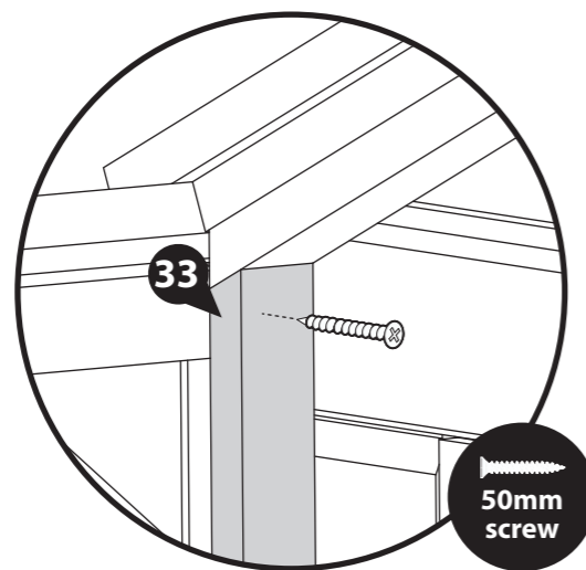
*Internal View*
