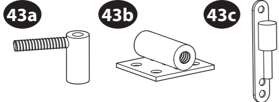
Adjustable Hinge QTY 6 PI-07-0209
