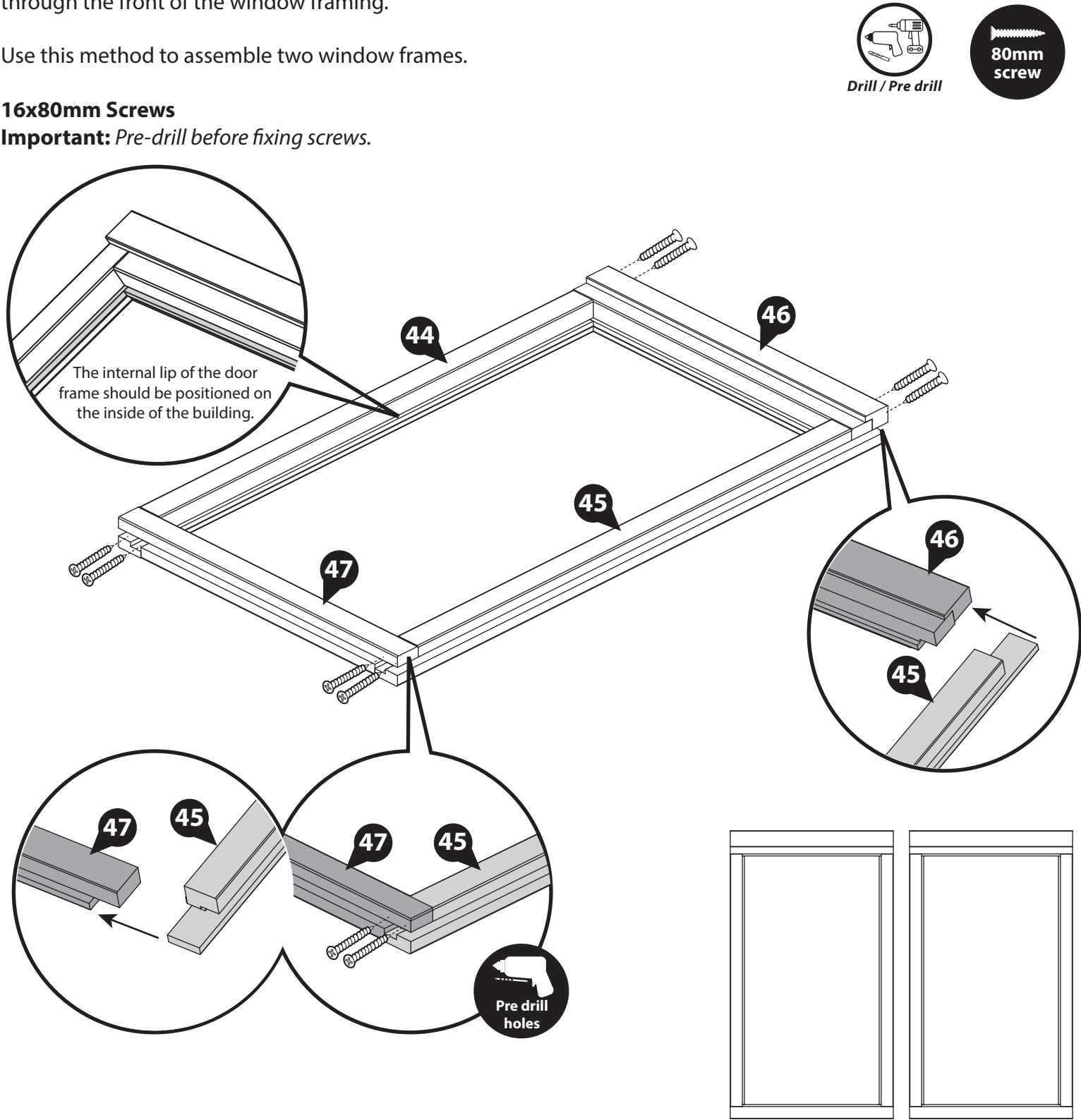
*Assembled frame front view*
