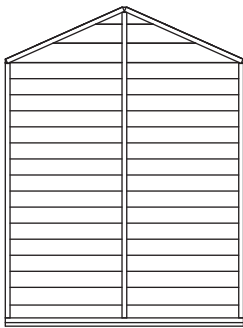
Back Gable QTY 1
