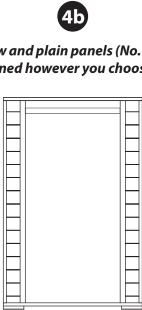
4ft Door Panel QTY 1 SU-01S21SHSD1180X1802-V1
