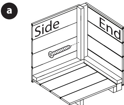
*Standard Panels*
