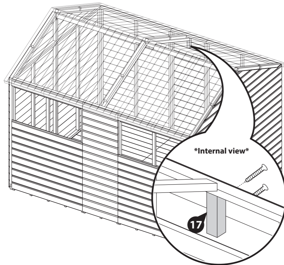
Truss Support Block is NOT required.
